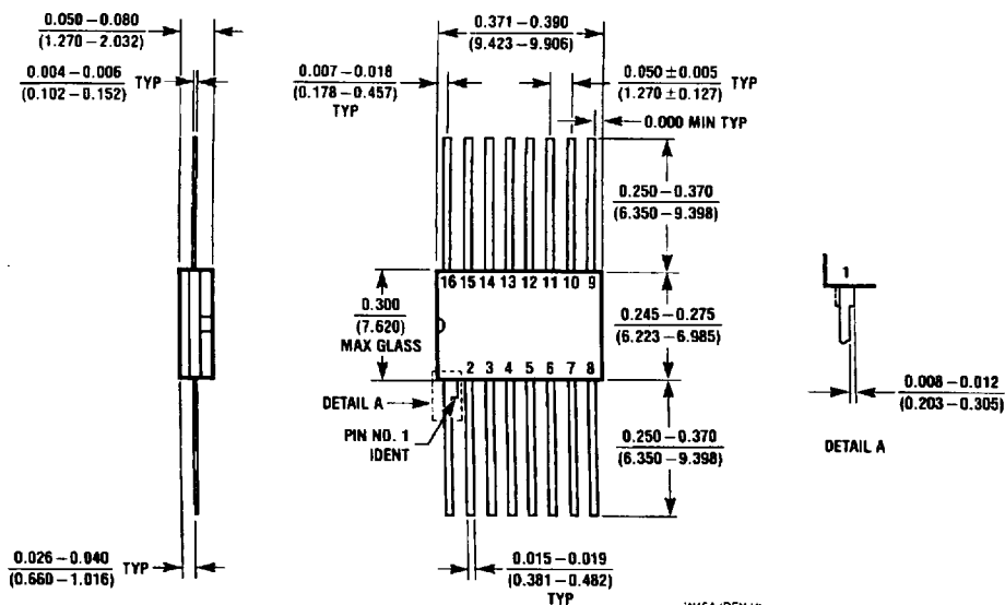
16-Lead Ceramic Flat Package (W) Order Number DM54LS503W NS Package Number W16A
