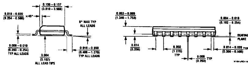
16-Lead Wide Small Outline Molded Package (M) Order Number DM74LS503WM NS Package Number M16B
