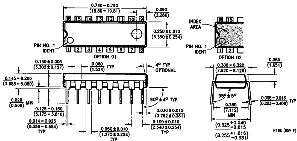
16-Lead Molded Dual-In-Line Package (N) Order Number DM74LS503N NS Package Number N16E
