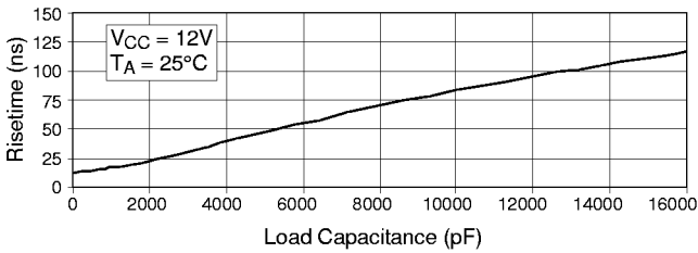
Figure 2: Gate(H) and Gate(L) Rise Time vs. Load Capacitance.
