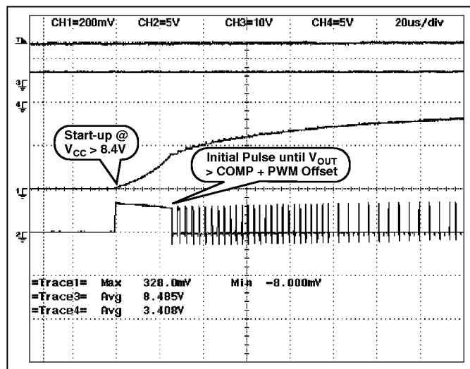
Figure 9: Normal Startup showing initial pulse followed by Soft Start (20μs/div).
