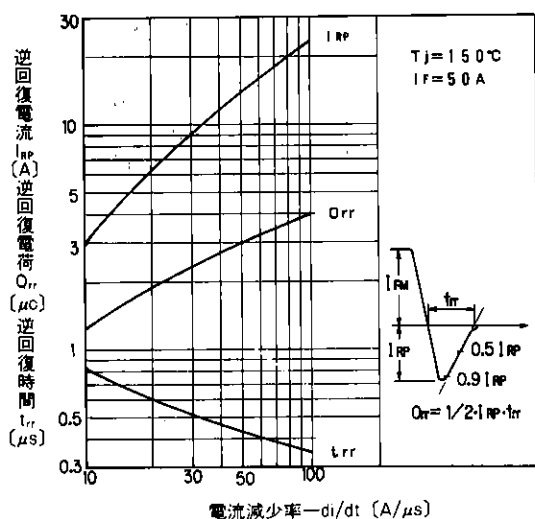
逆回復特性 Reverse Recovery Charge
