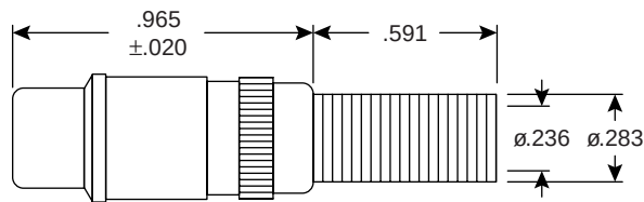
Dimensions (In.)
