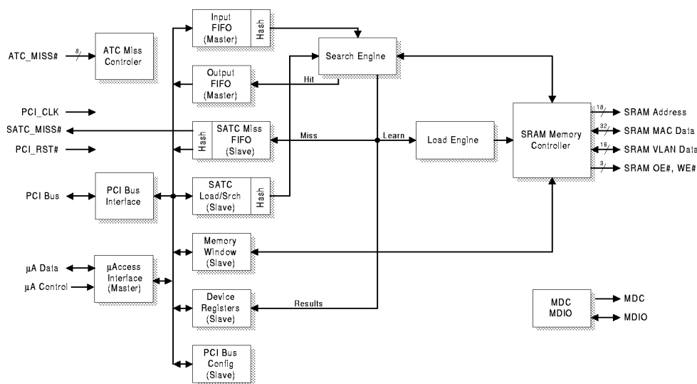
Figure 1: LS105 Functional Block Diagram
