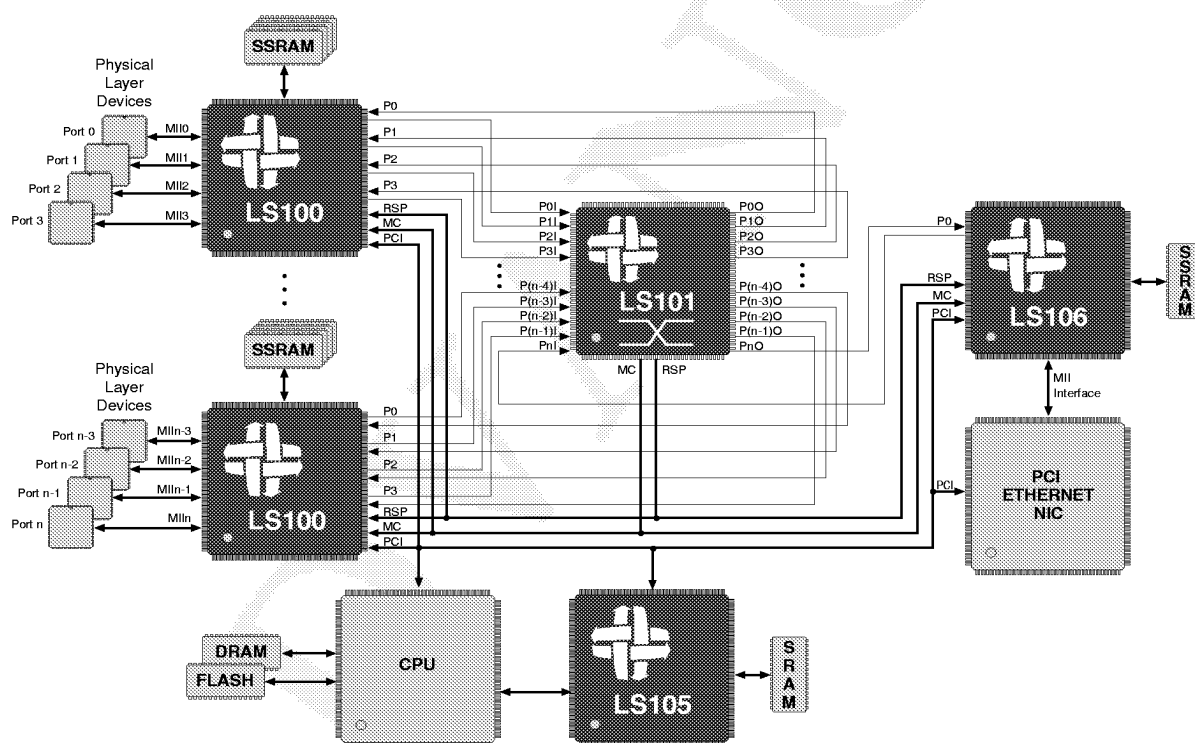
Figure 2: The LS Family System Block Diagram
