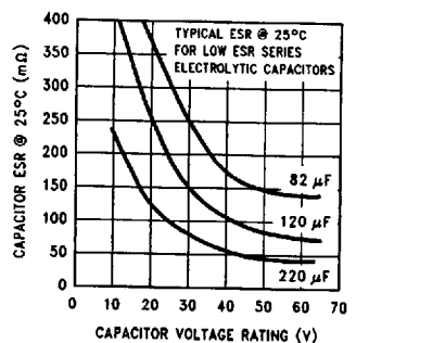
FIGURE 16. Capacitor ESR vs Capacitor Voltage Rating (Typical Low ESR Electrolytic Capacitor)
