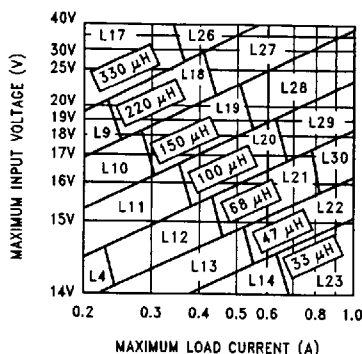
FIGURE 6. LM2598-12
