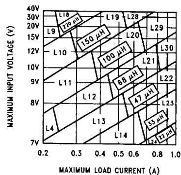
FIGURE 5. LM2598-5.0
