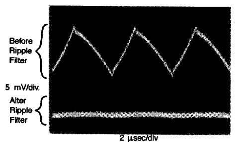
FIGURE 19. Post Ripple Filter Waveform
