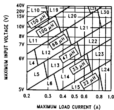
FIGURE 4. LM2598-3.3
