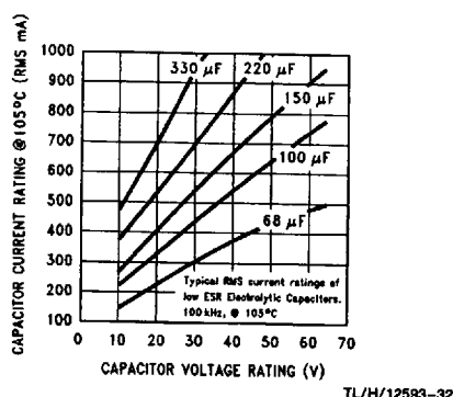
FIGURE 15. RMS Current Ratings for Low ESR Electrolytic Capacitors (Typical)
