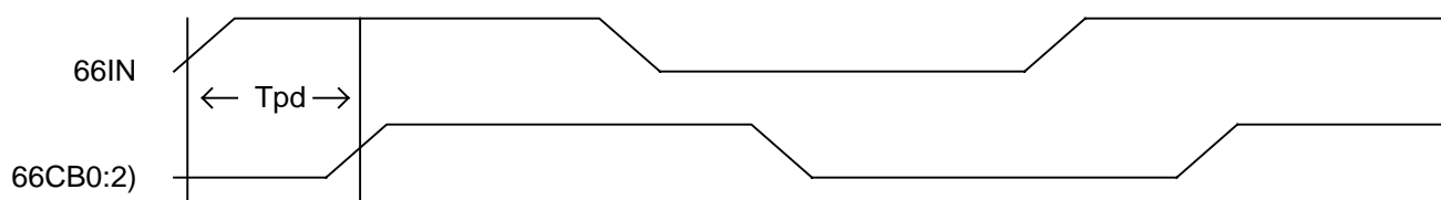
66IN to 66B(0:2) Output Delay Figure
