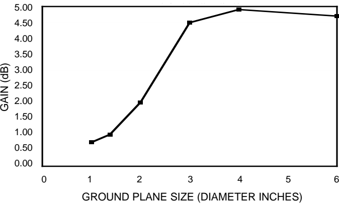
ANTENNA ZENITH GAIN vs. GROUND PLANE SIZE GPS MICRO PATCH ANTENNAS
