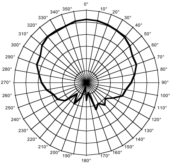
Typical Antenna Pattern (10 dB/division)
