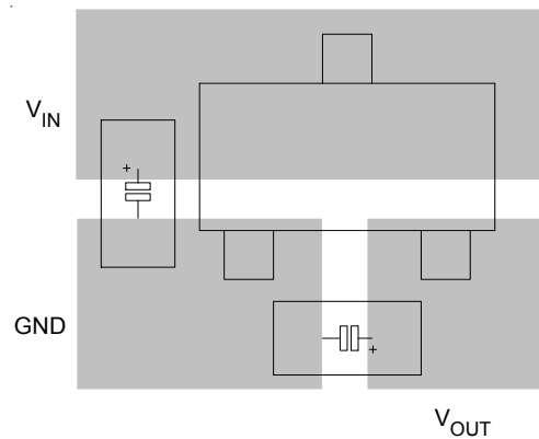
SOT-23 Board Layout
