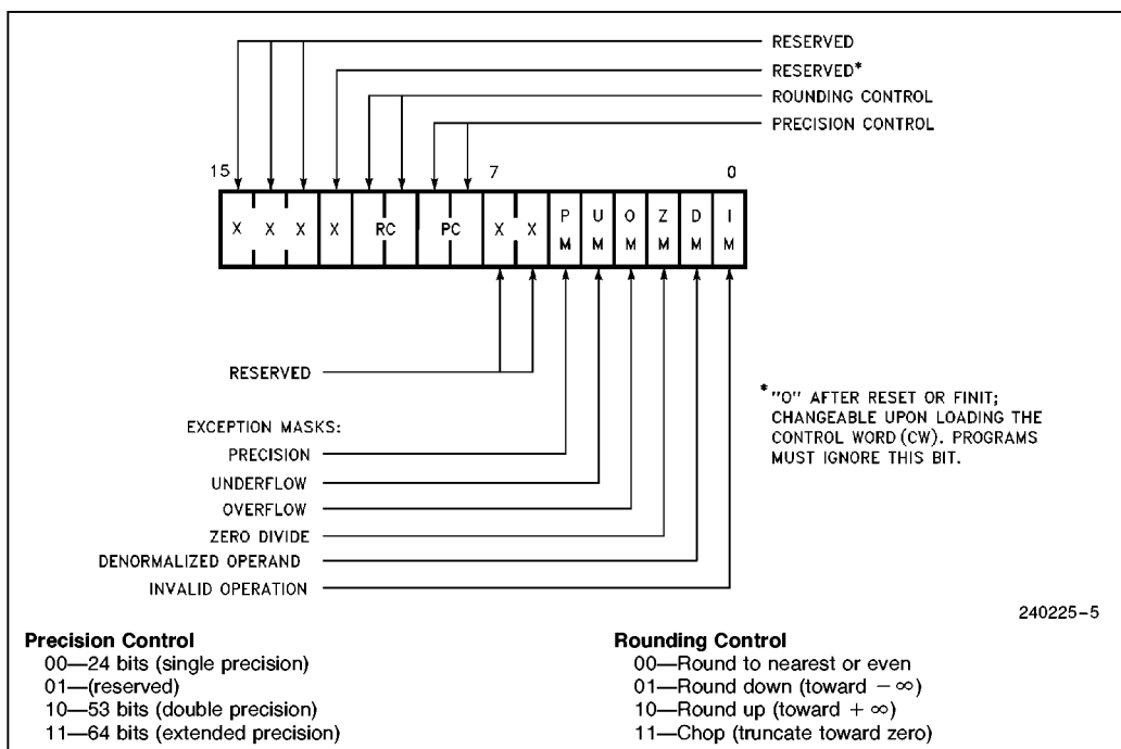
Figure 3-3. Control Word
