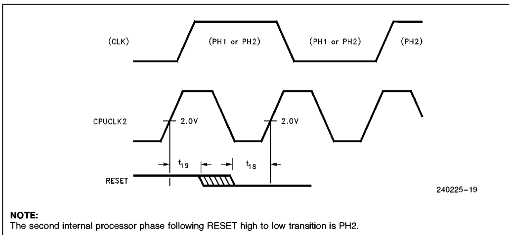
Figure 7-5. RESET Signal
