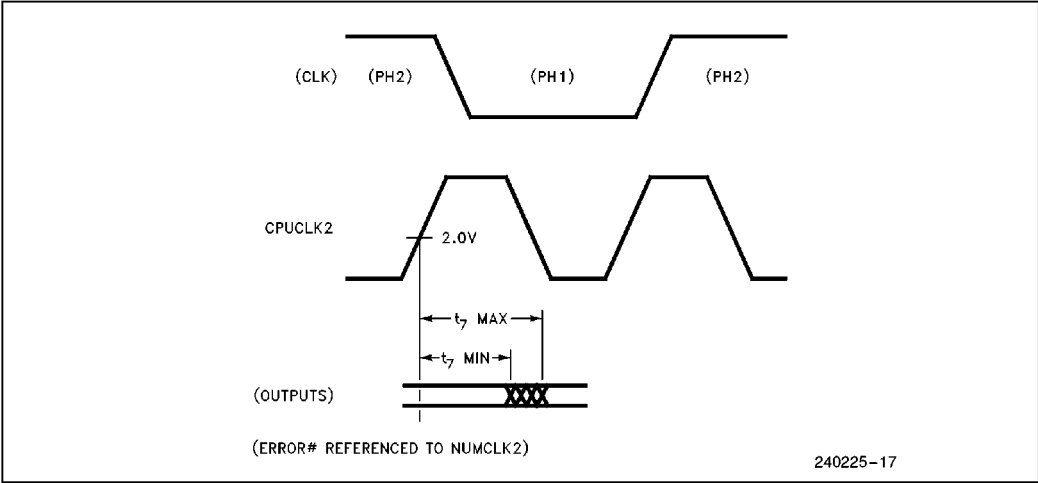
Figure 7-3. Output Signals
