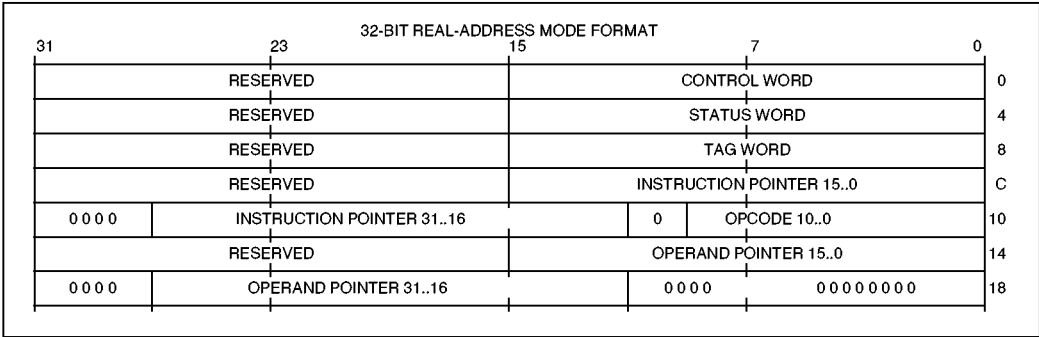
Figure 3-7. Instruction and Data Pointer Image in Memory, 32-Bit Real-Mode Format
