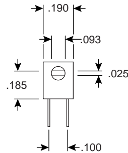
Dimensions (In.)
