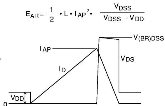
Avalanche Test Circuit and Waveform
