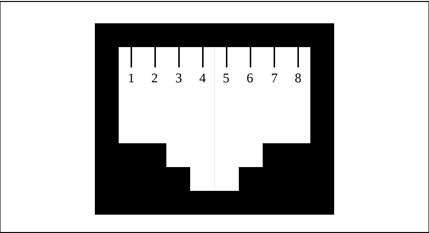
Figure 2-5. Front View of the RJ-45 Connector
