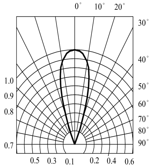
RADIATION DIAGRAM
