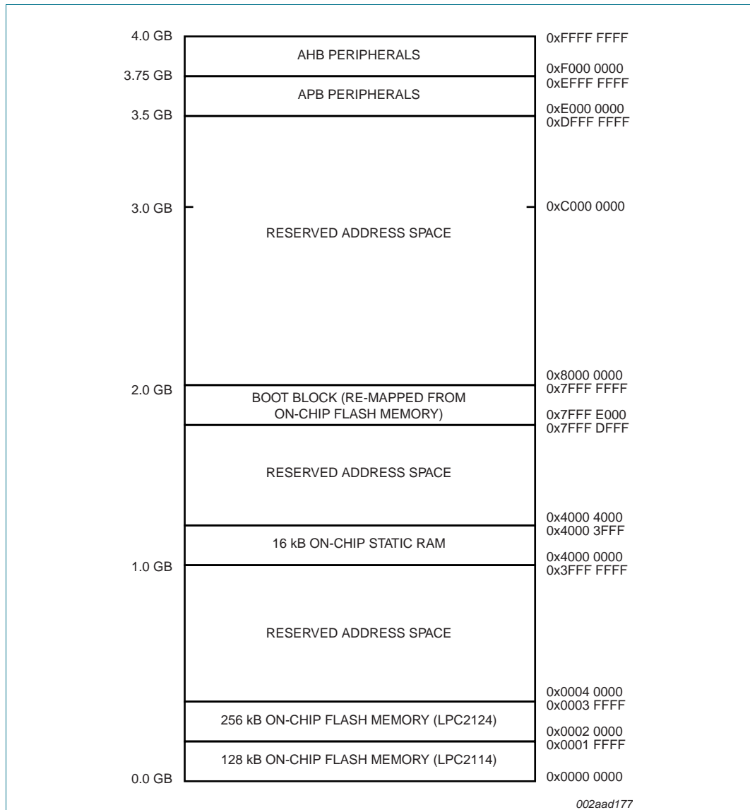
Fig 3. LPC2114/2124 memory map
