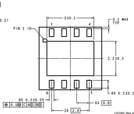
8 Lead LLP Surface Mount Package NS Package Number LDC08A
