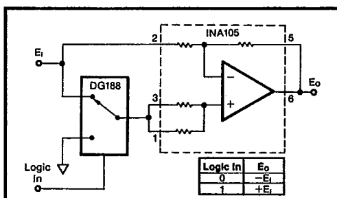
FIGURE 26. Digitally Controlled Gain of \pm 1 Amplifier.
