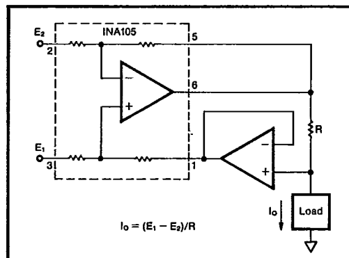
FIGURE 24. Differential Input Voltage-to-Current Converter for Low I_{0\text{ur}} .
