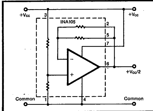
FIGURE 11. Pseudoground Generator.
