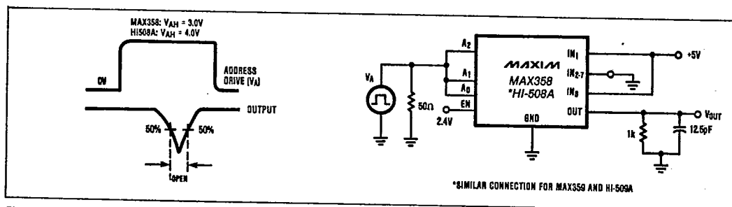
Figure 2. Break Before Make Delay ( t_{OPEN} )
