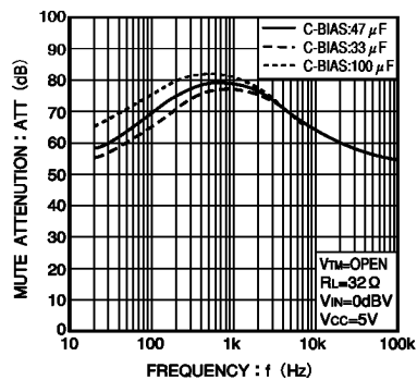
Fig.12 MUTE attenuation vs. frequency
