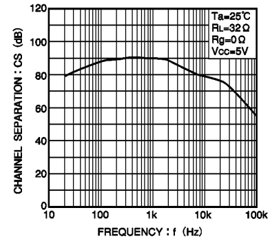
Fig.11 Channel separation vs. frequency
