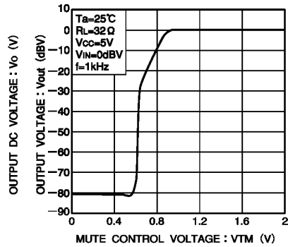
Fig.5 Output voltage vs. MUTE control voltage
