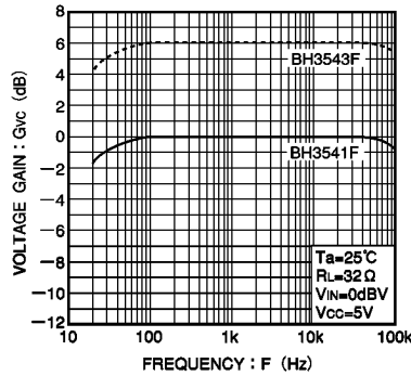
Fig.6 Voltage gain vs. frequency
