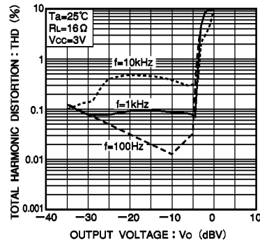
Fig.10 Total harmonic distortion vs. output voltage (IV)
