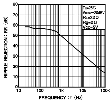
Fig.13 Ripple rejection vs. frequency
