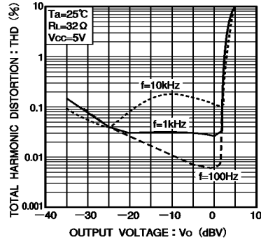
Fig.7 Total harmonic distortion vs. output voltage (I)
