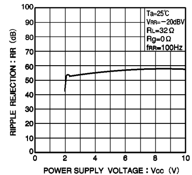
Fig.14 Ripple rejection vs. power supply voltage
