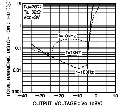
Fig.8 Total harmonic distortion vs. output voltage (II)
