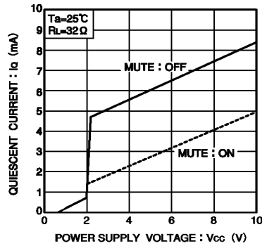
Fig.3 Quiescent current vs. power supply voltage
