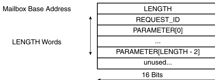
Figure 9. Request Notification Message Format
