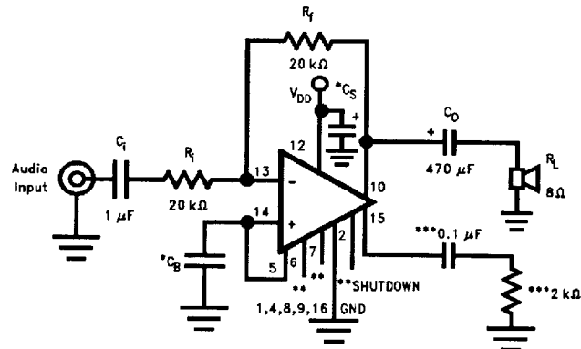
FIGURE 3. Single-Ended Amplifier with A_V = -1
