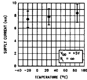
Supply Current Distribution vs Temperature
