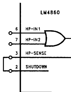
FIGURE 4. HP-SENSE Pin to SHUTDOWN Pin Connection
