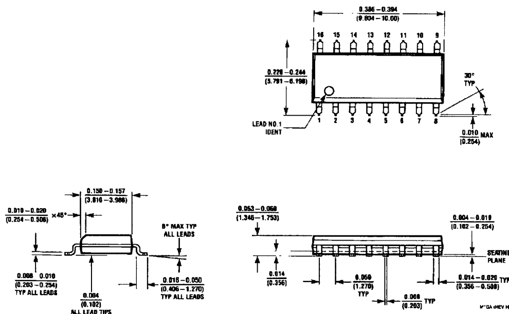
Small Outline Package (M) Order Number LM4860M NS Package Number M16A
