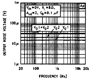
LM4860 Noise Floor vs Frequency
