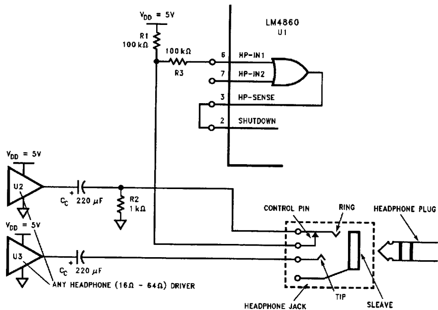
FIGURE 5. Typical Headphone Control Input Circuitry
