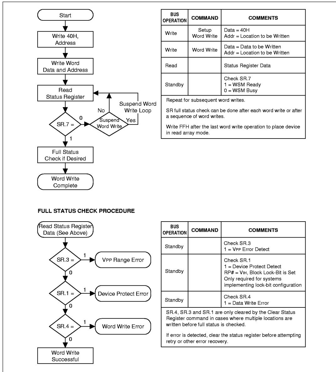
Fig. 4 Automated Word Write Flowchart
