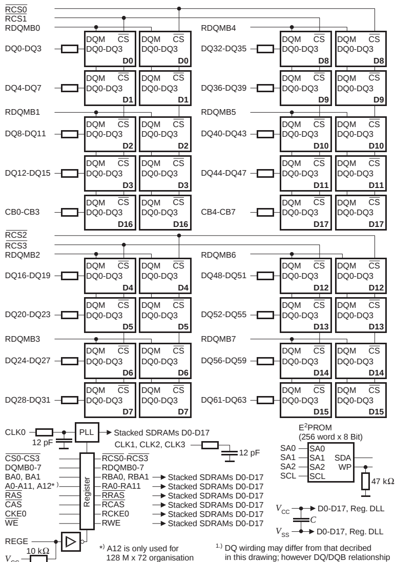
Block Diagram: Two Bank 128M x 72 SDRAM DIMM Modules HYS 72V128220GR Using Stacked x4 Organized SDRAMs
