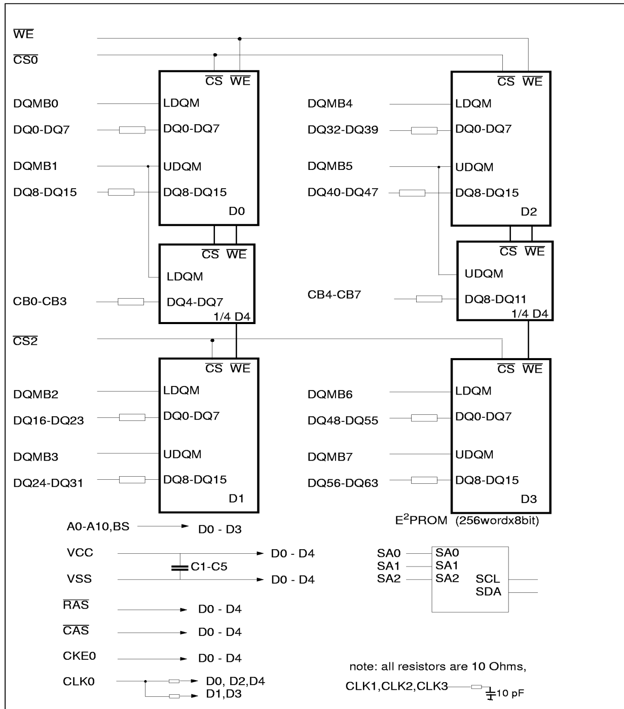
Block Diagram for 1M x 72 SDRAM - DIMM module
