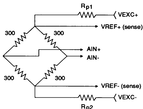
Figure 3. Six-Wire Bridge
