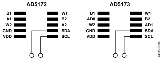
Figure 48. Recommended AD5172/AD5173 PCB Layout. The SCL and SDA pads allow pogo pins to be inserted so that signals can be communicated through the parallel port for programming (Figure 47).
