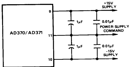
Figure 2. Power Supply Decoupling
