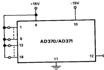
Figure 3. Burn-In Circuit
