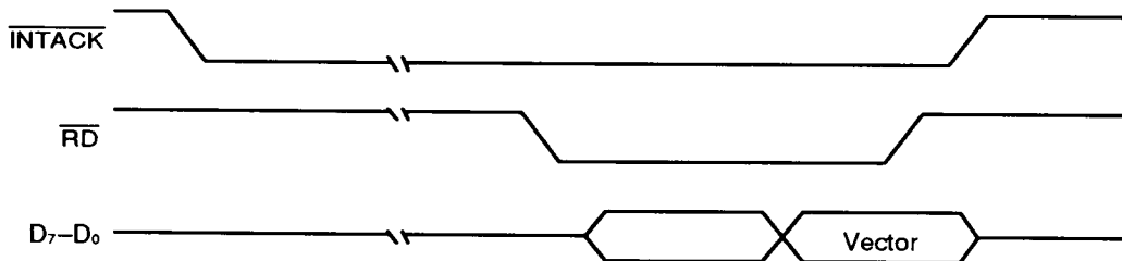
Figure 12. Interrupt Acknowledge Cycle Timing
