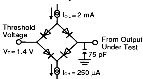
Standard Test Dynamic Load Circuit
