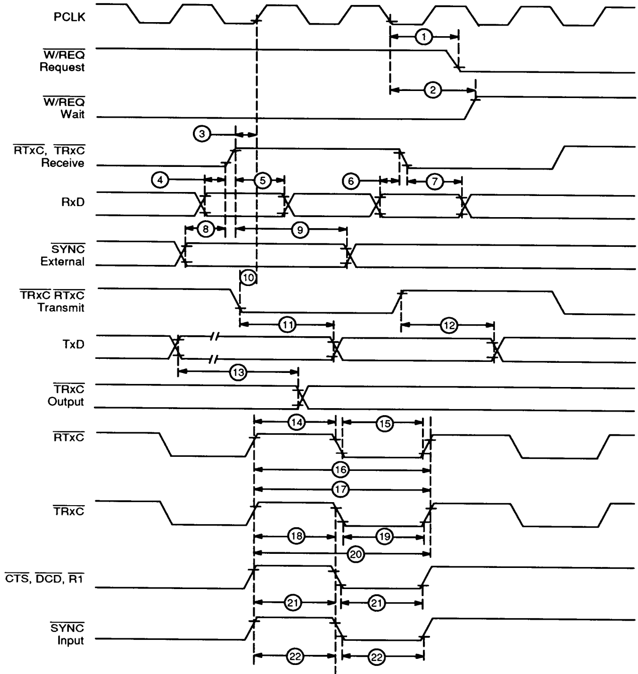
Figure 19. General Timing
