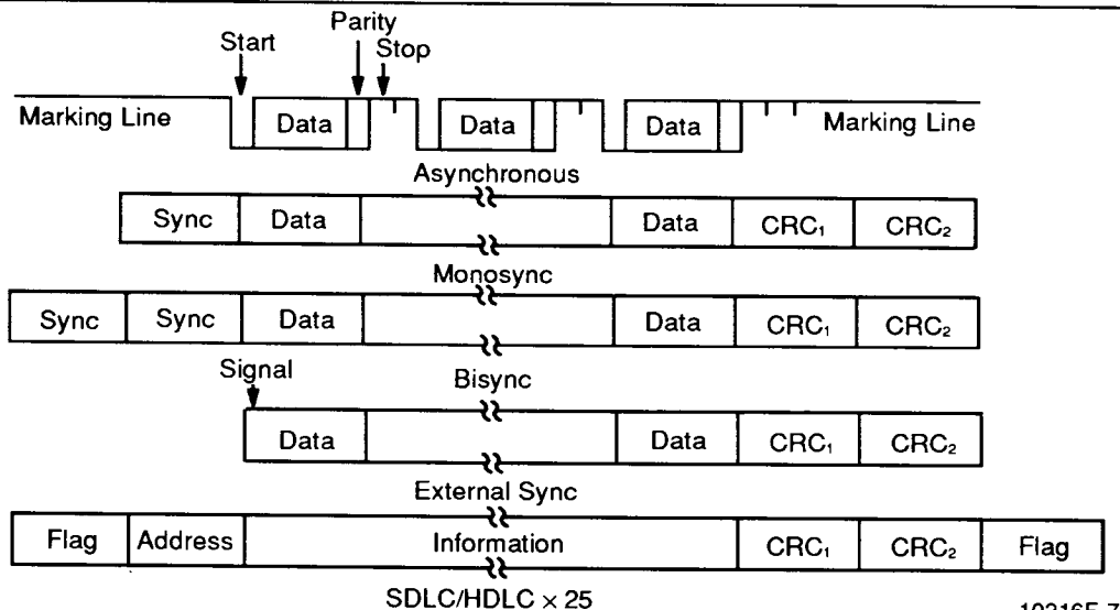
Figure 3. SCC Protocols
