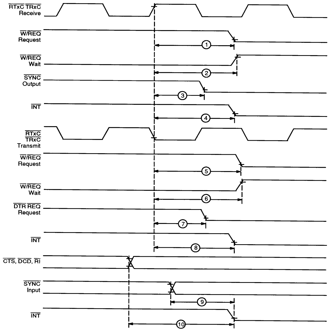
Figure 20. System Timing
