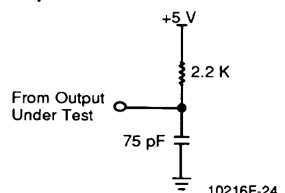
Open-Drain Test Load
