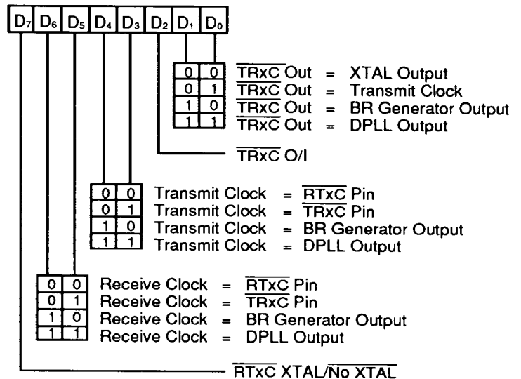
Figure 9. Write Register Bit Functions (continued)
