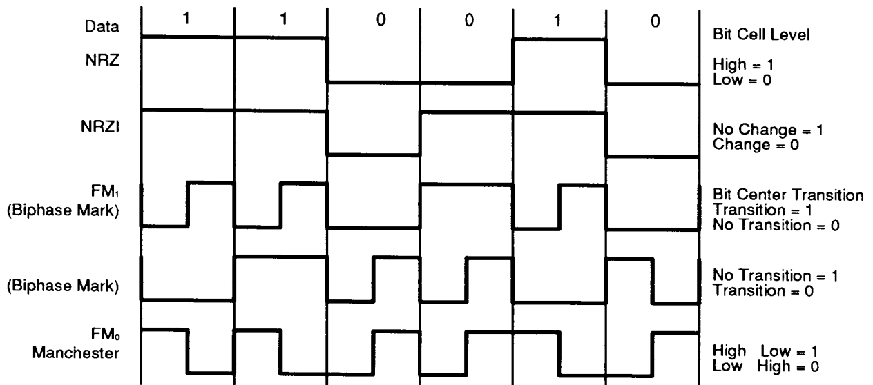
Figure 6. Data Encoding Methods
