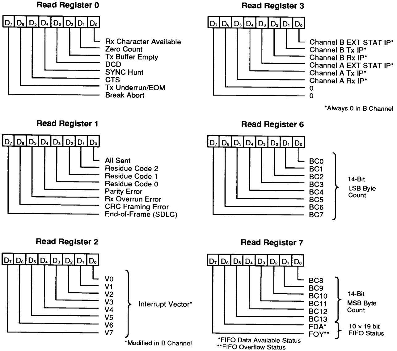
Figure 8. Read Register Bit Functions
