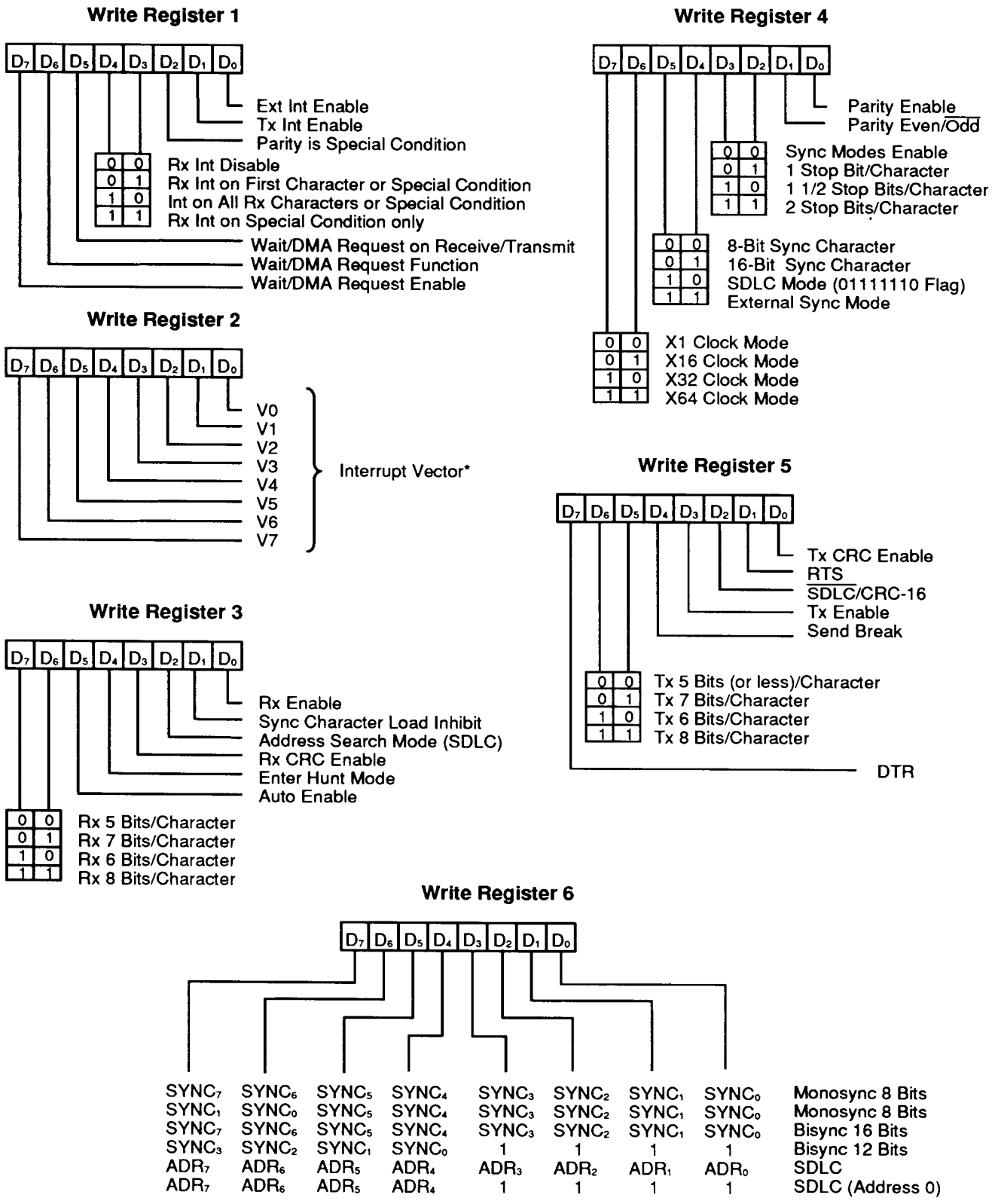
Figure 9. Write Register Bit Functions (continued)
