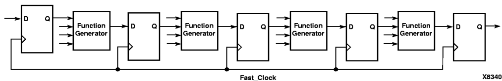
Figure 4-13 After Pipelining
