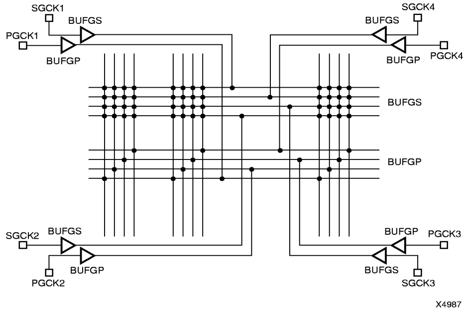
Figure 4-1 Global Buffer Routing Resources (XC4000E, Spartan)
