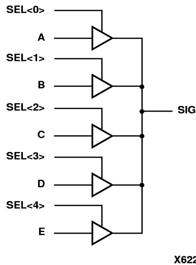
Figure 4-11 5-to-1 MUX Implemented with BUFTs
