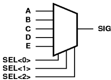
Figure 4-10 5-to-1 MUX Implemented with Gates
