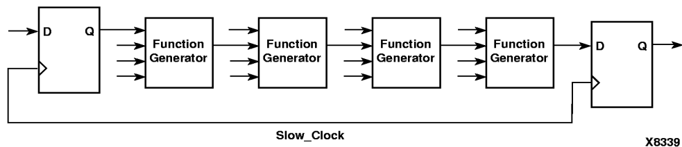
Figure 4-12 Before Pipelining
