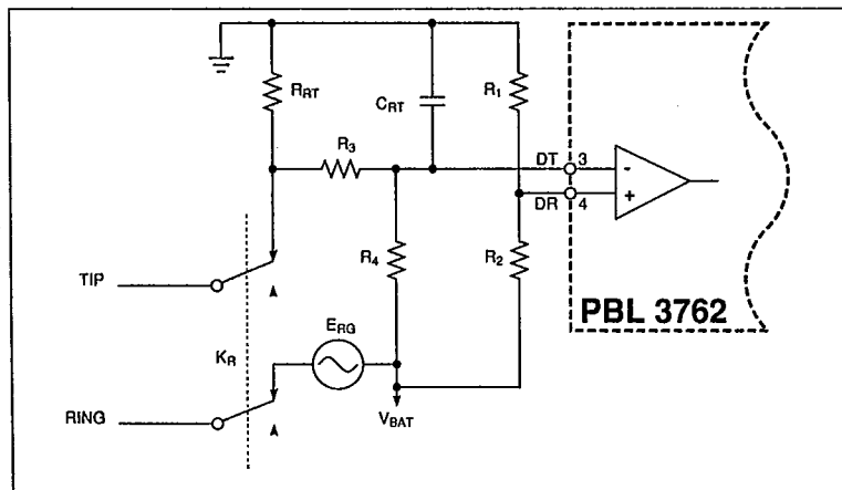
Figure 18. Ring trip network.
