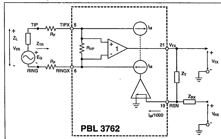
Figure 7. Simplified ac transmission circuit.
