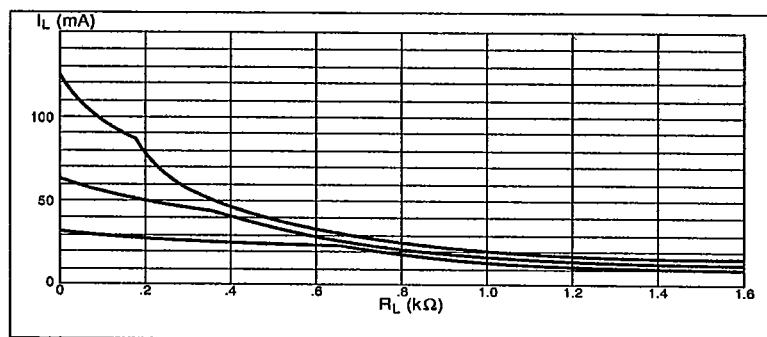
Figure 14. Examples of PBL 3762 loop feed. R_{SG} \rightarrow \infty , V_{Batt} = -28\text{V} .
