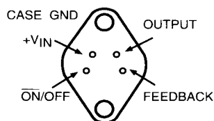
4-LEAD TO-3 (K)
