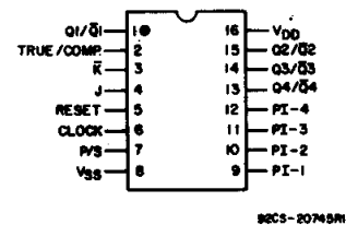
TERMINAL DIAGRAM Top View
