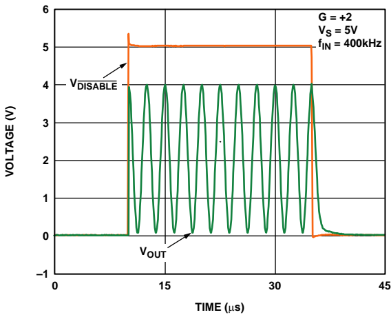
Figure 23. Enable/Disable Time
