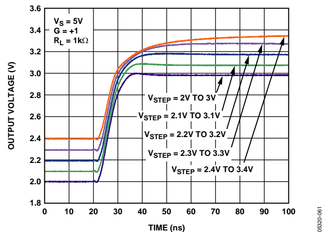
Figure 39. Pulse Response, Input Headroom Limits
