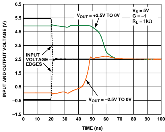
Figure 40. Overload Recovery
