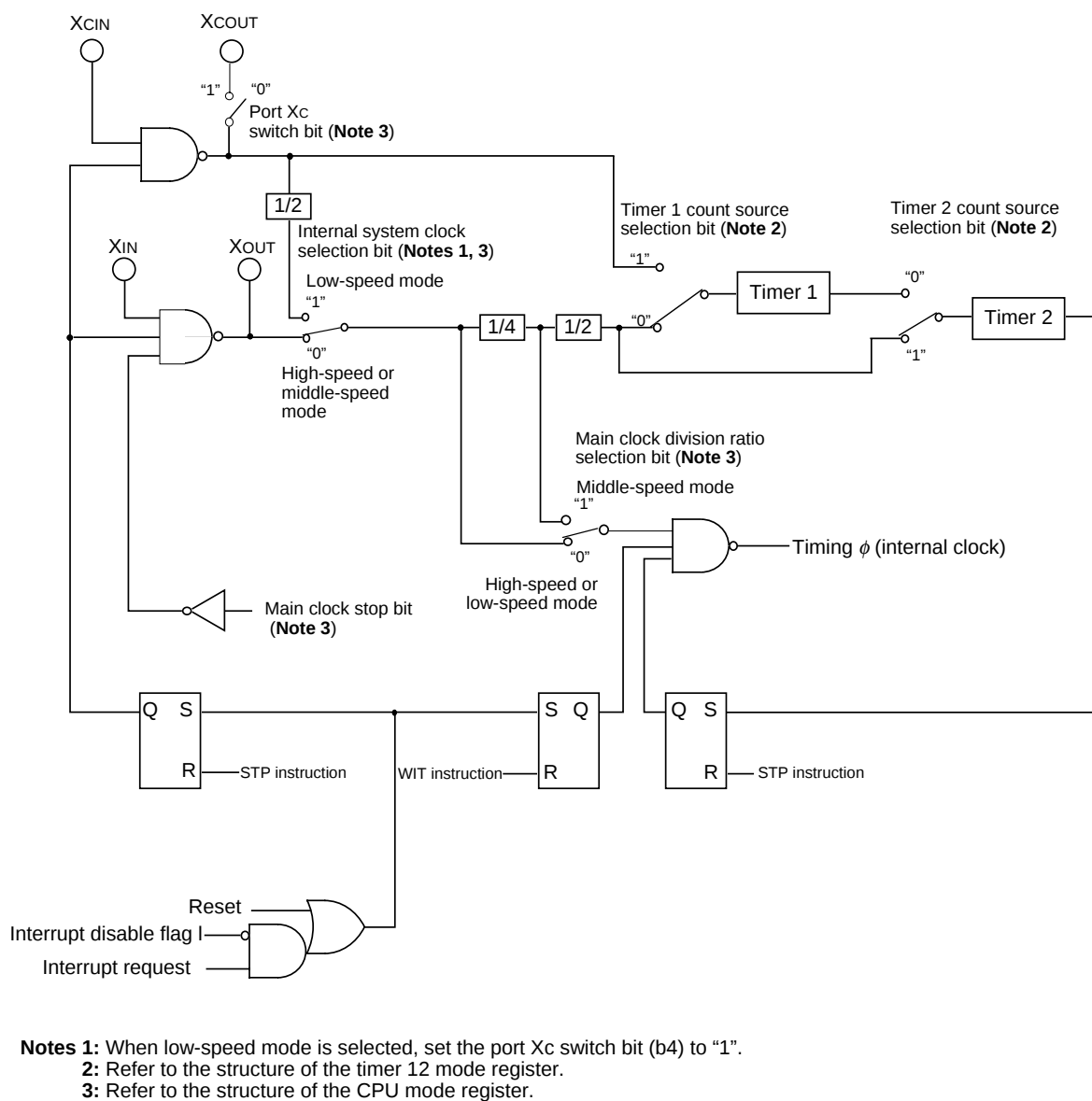
Fig. 73 Clock generating circuit block diagram
