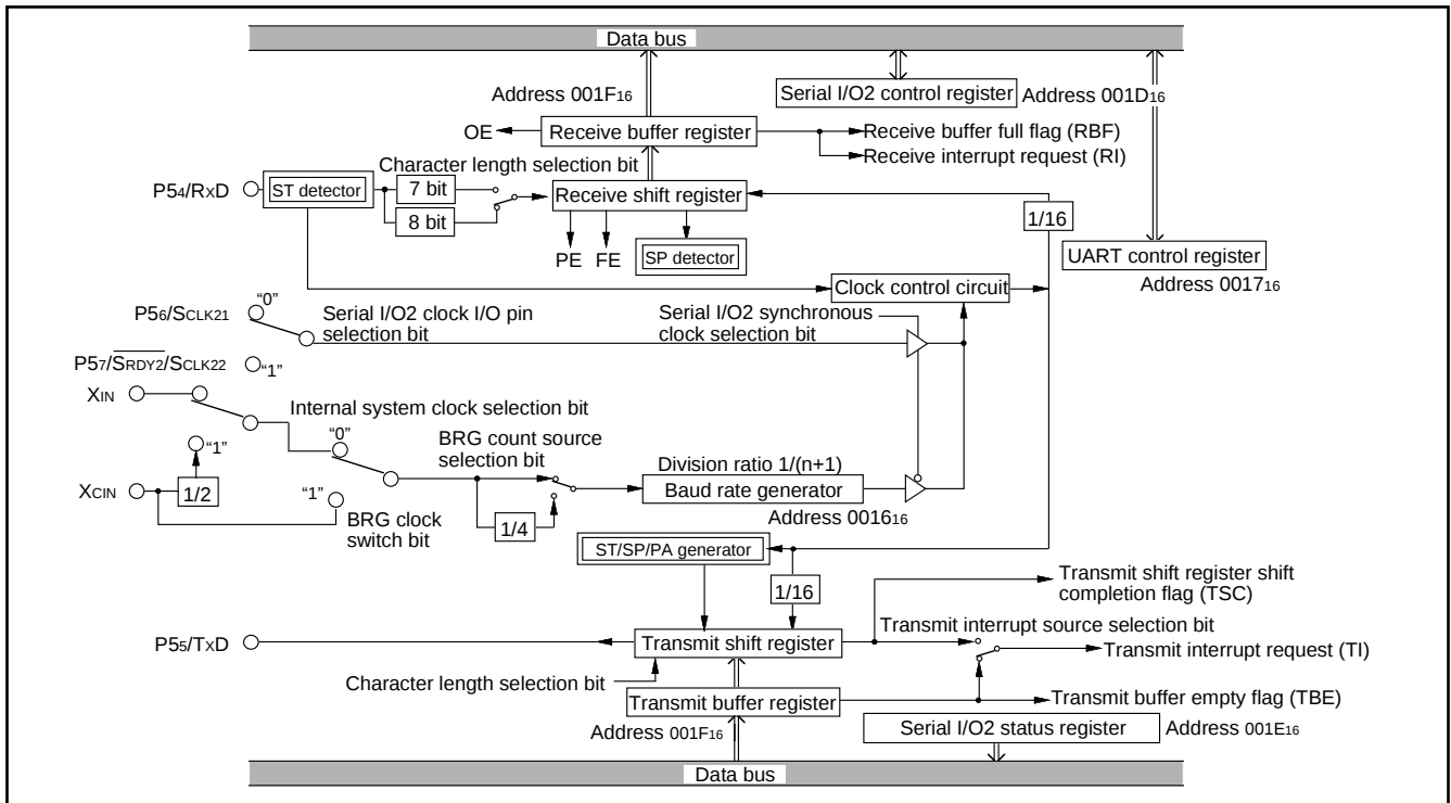
Fig. 39 Block diagram of UART serial I/O2
