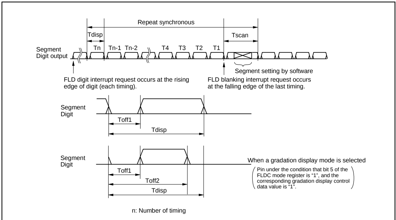
Fig. 51 FLDC timing
