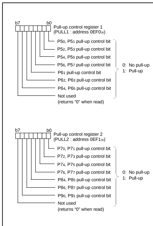
Fig. 10 Structure of pull-up control registers (PULL1 and PULL2)
