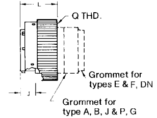
Crimp KPSE06/MS3126
