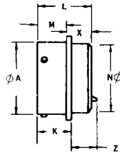
Solder KPT02/MS3112
