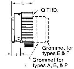
Crimp KPSE08
