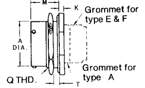
Crimp KPSE07/MS3124
