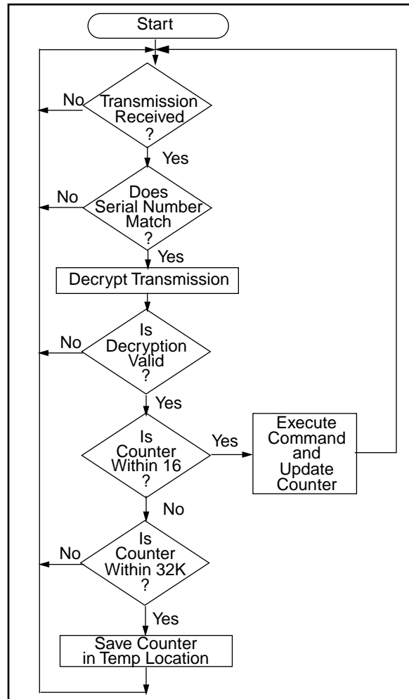
FIGURE 6-3: DECODER OPERATION
