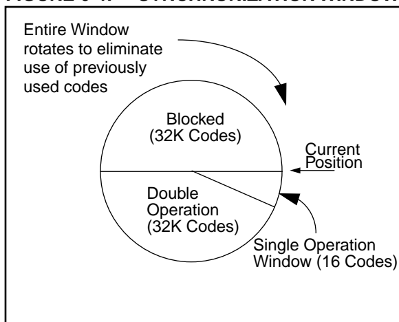
FIGURE 6-4: SYNCHRONIZATION WINDOW
