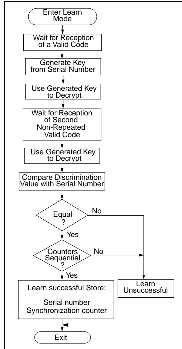
FIGURE 6-2: LEARN SEQUENCE
