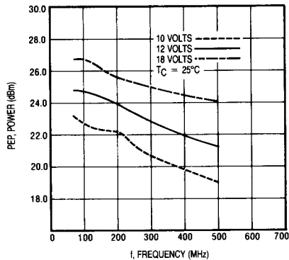
Figure 6. Peak Envelope Power versus Voltage
