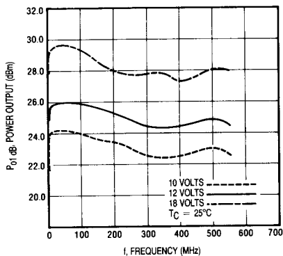
Figure 3. 1 dB Gain Compression versus Voltage
