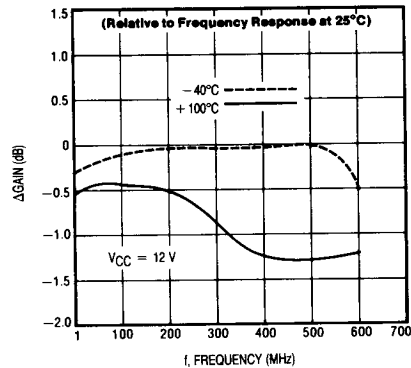
Figure 2. Relative Power Gain versus Temperature
