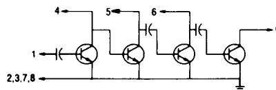
Figure 11. External Connections
