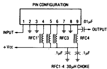
Figure 12. External Connections
