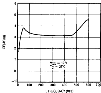
Figure 8. Group Delay versus Frequency
