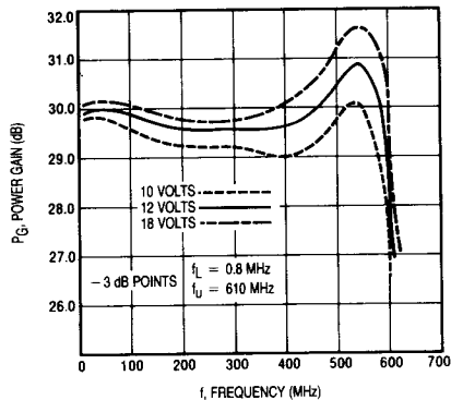
Figure 1. Power Gain versus Frequency
