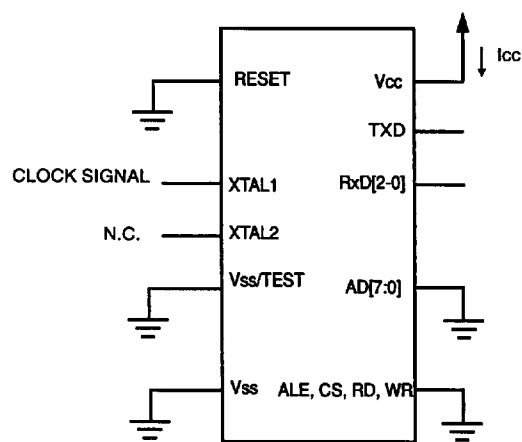
Figure 32. I CC
