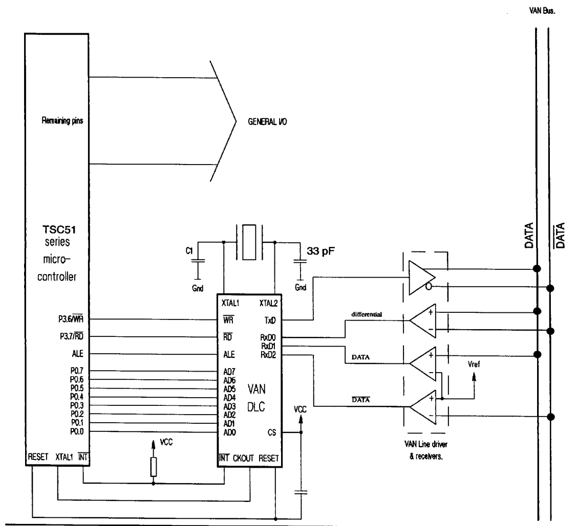
Figure 3. Typical Application
