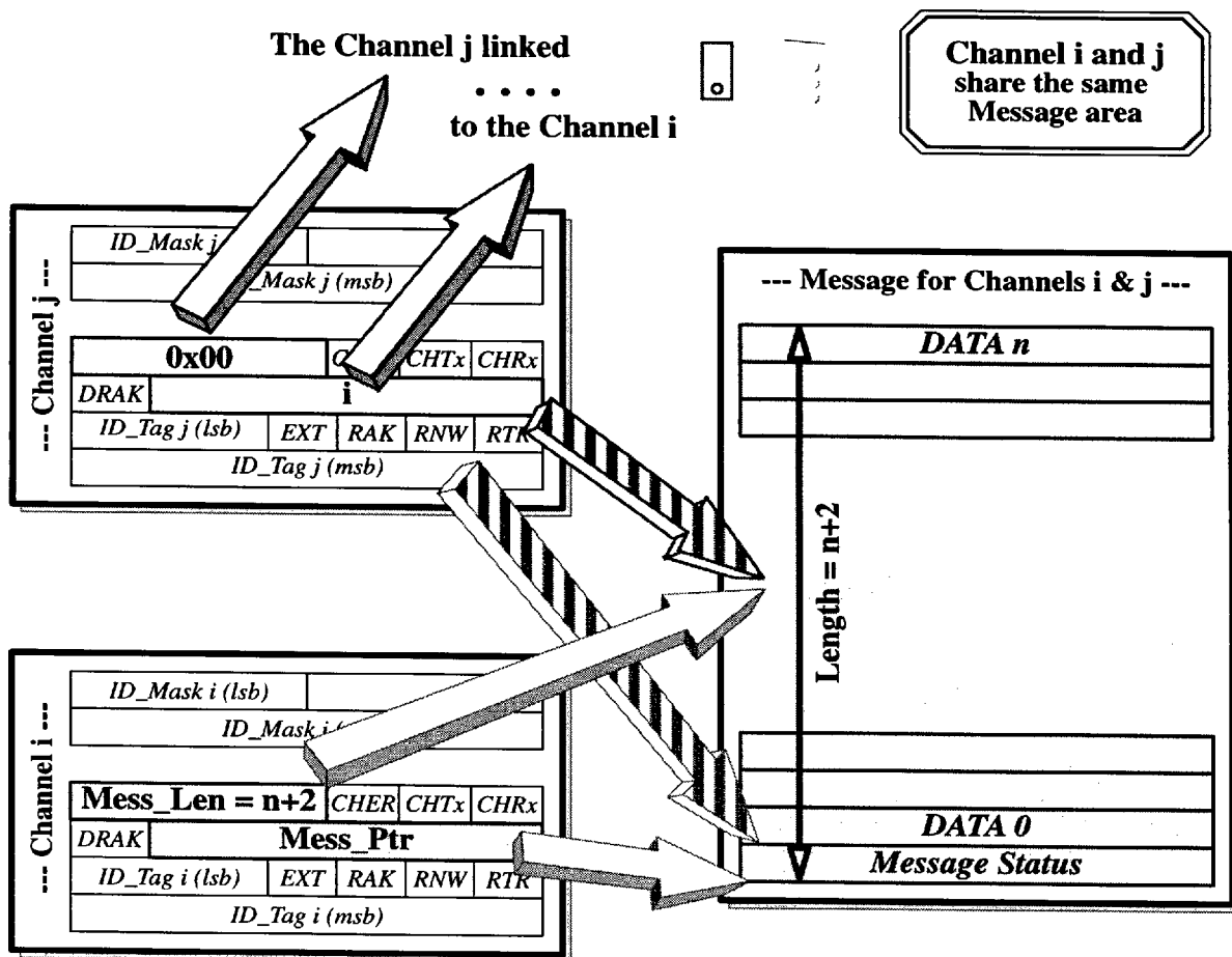
Figure 31. Linkage mechanism
