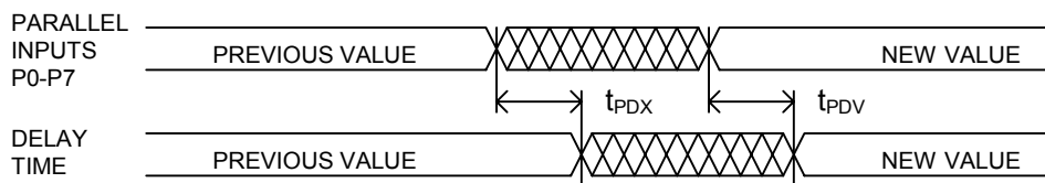
Figure 2: Non-latched parallel mode (MD=1, AE=1)
