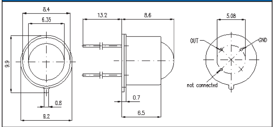
Figure 4. Package Dimensions
