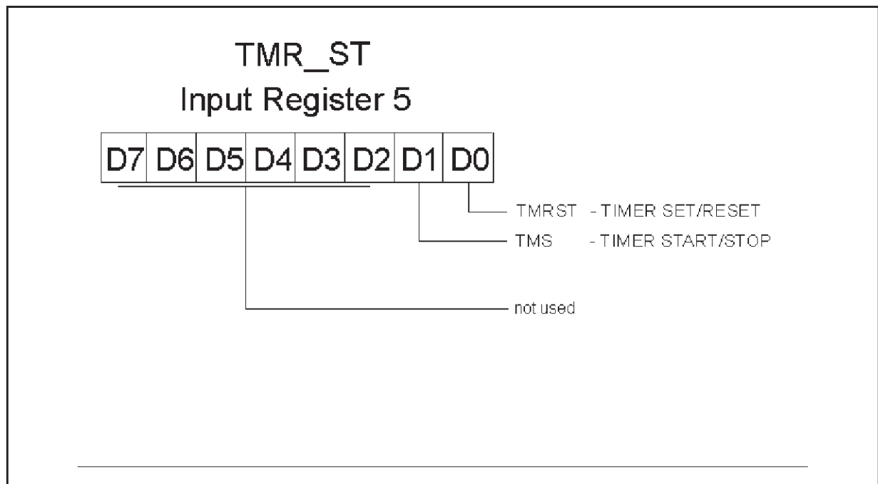
Figure 2.6. TMR_ADC_ST Registers
