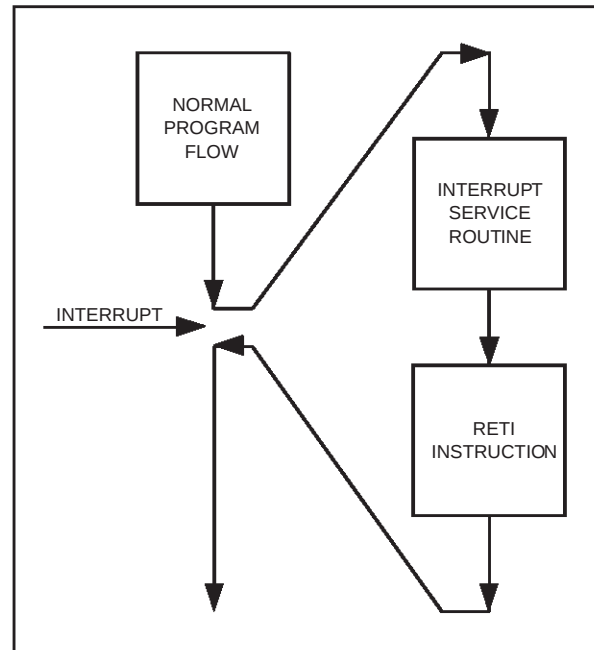
Figure 4.1. Interrupt Flow
