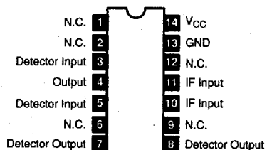
NTE1096 14-Lead DIP, See Diag. 268 High Frequency Wide Band Amp/ Phase Detector
