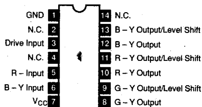
NTE1099 14-Lead DIP, See Diag. 247 Chroma Demod, V_{CC} = 28V
