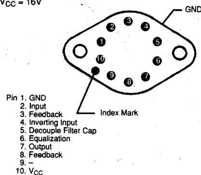
NTE1098 (Bottom View) 10-Lead TO3, See Diag. 198 Audio Power Amp, 5W, V_{CC} = 16V
