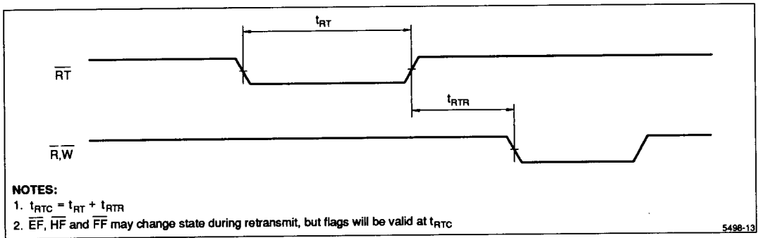
Figure 14. Retransmit Timing
