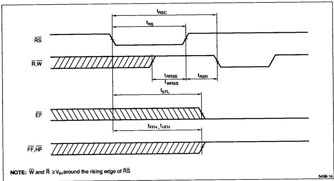
Figure 5. Reset Timing
