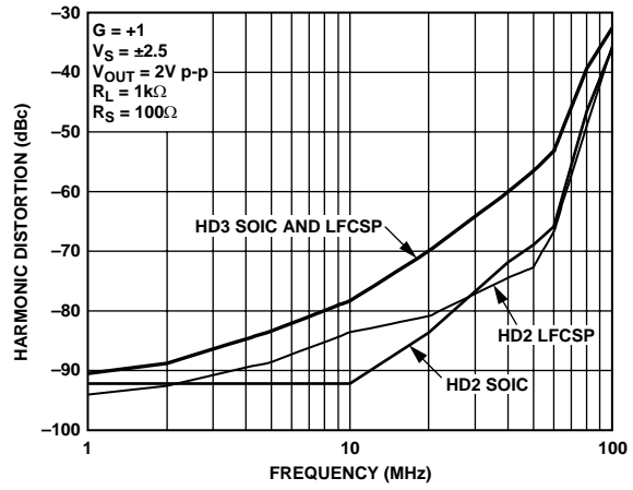
Figure 28. Harmonic Distortion vs. Frequency for Various Packages
