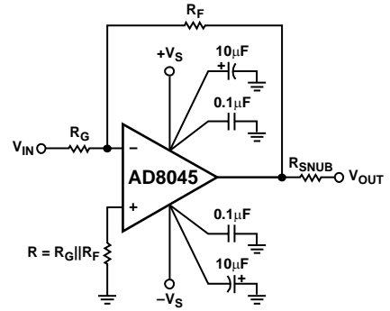
Figure 62. Inverting Configuration
