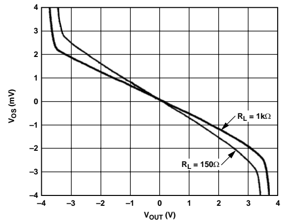
Figure 59. Input Offset Voltage vs. Output Voltage for Various Loads
