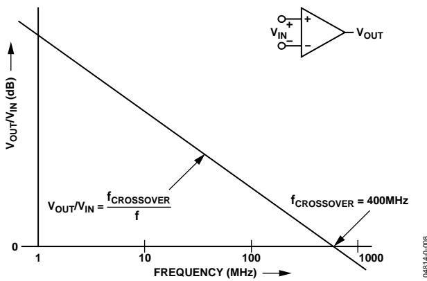
Figure 63. Open-Loop Response
