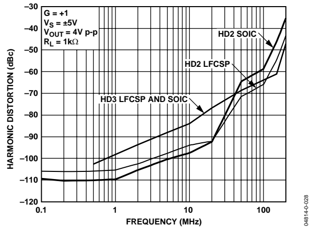
Figure 18. Harmonic Distortion vs. Frequency for Various Packages
