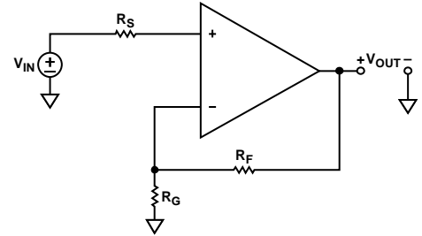
Figure 64. Noninverting Configuration
