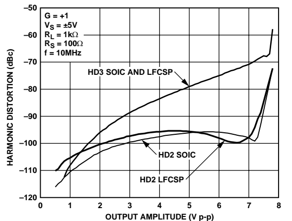
Figure 24. Harmonic Distortion vs. Output Voltage for Various Packages
