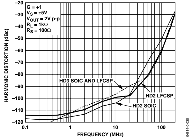
Figure 17. Harmonic Distortion vs. Frequency for Various Packages
