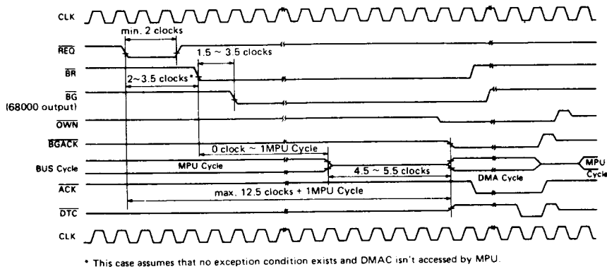
Figure 13 DMAC Bus Arbitration Timing
