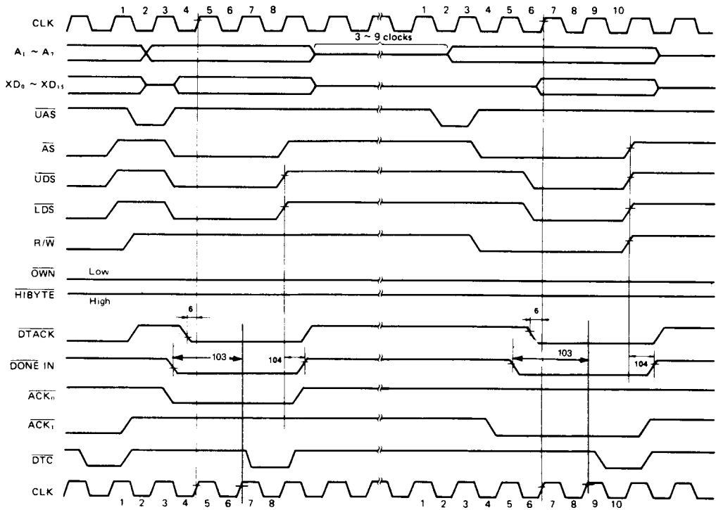
Figure 8 AC Electrical Waveforms – \overline{DONE} Input
