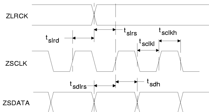
Figure 4. ZV PORT
