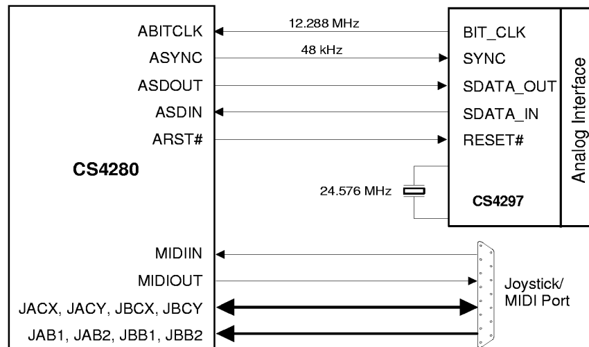
Figure 8. AC '97 Codec Connection Diagram
