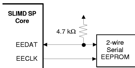
Figure 10. External EEPROM Connection
