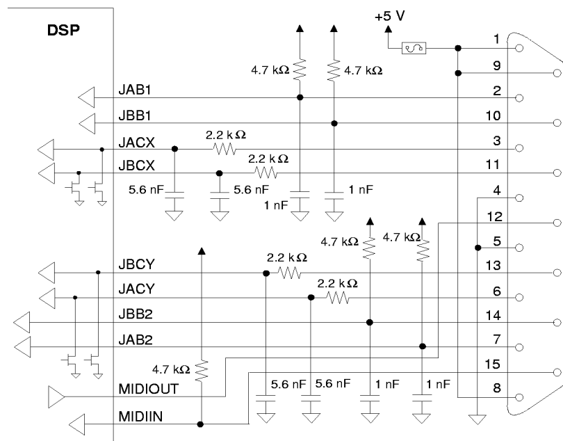
Figure 9. Joystick Logic
