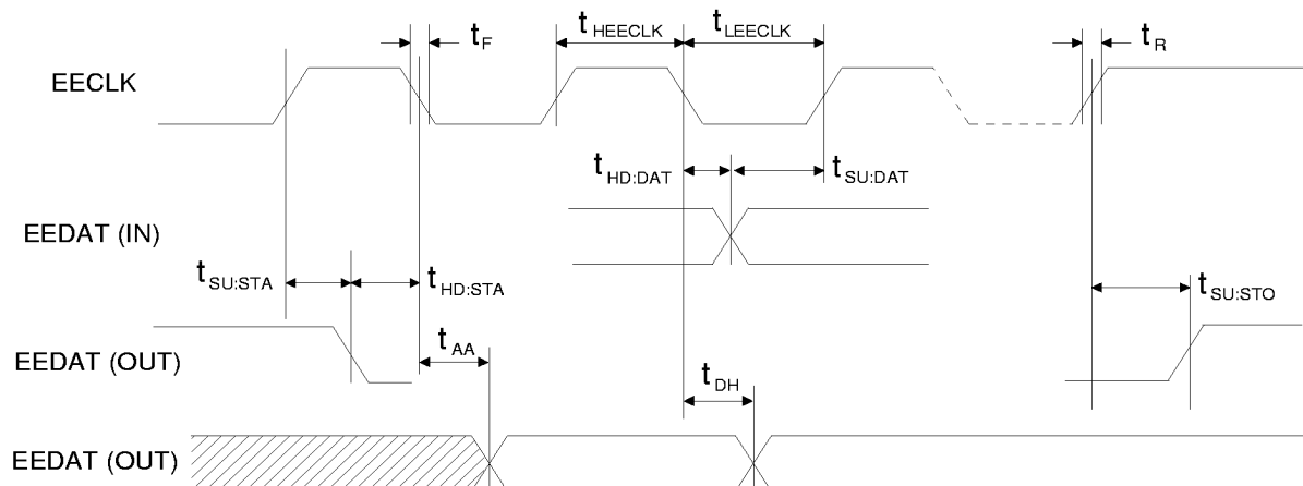
Figure 5. EEPROM Timing
