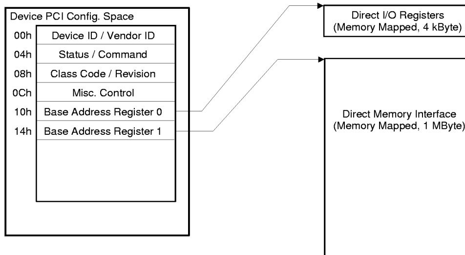
Figure 7. Host Interface Base Address Registers
