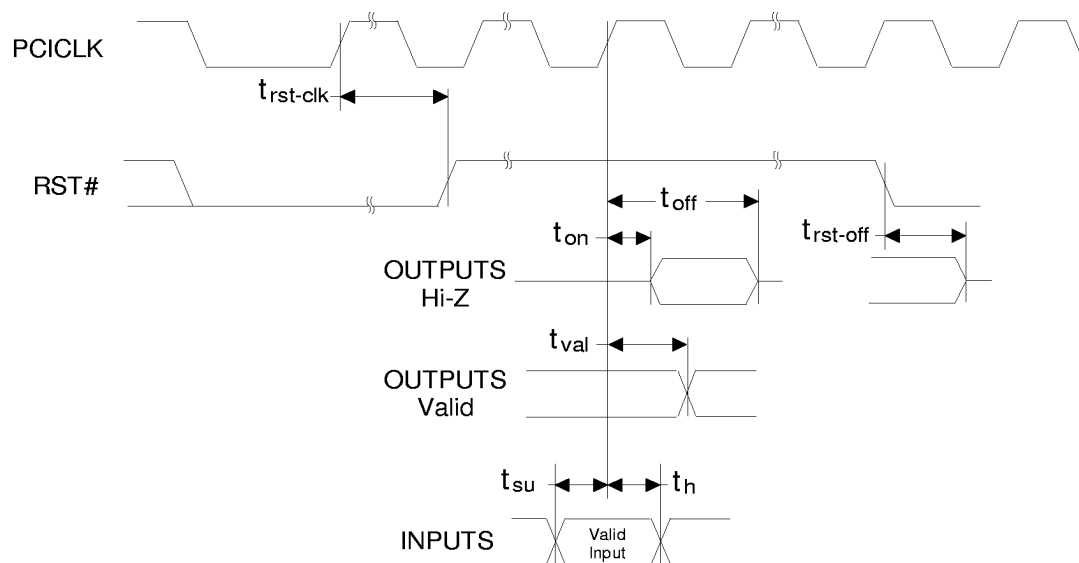
Figure 2. PCI Timing Measurement Conditions
