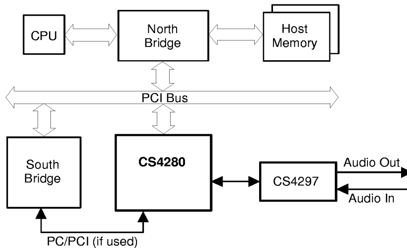
Figure 6. AC '97 Codec Interface
