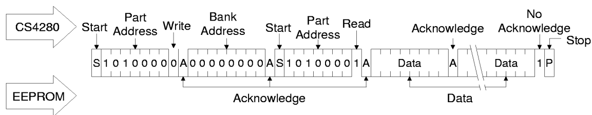
Figure 11. EEPROM Read Sequence
