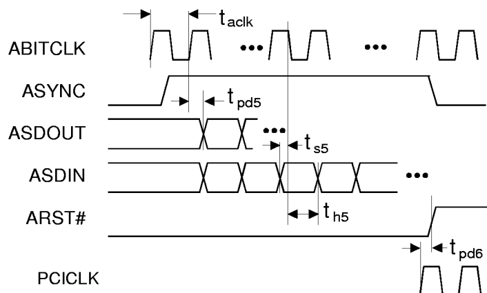
Figure 3. AC '97 Configuration Timing Diagram
