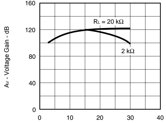
V^+ - Power Supply Voltage - V ( V^- = \text{GND} )
