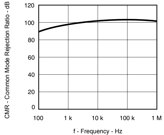
CMR vs. f
