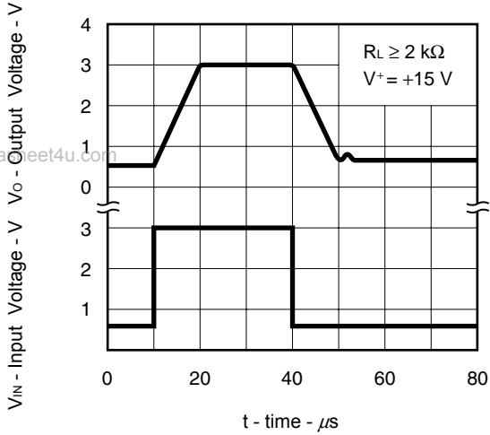
PULSE RESPONSE
