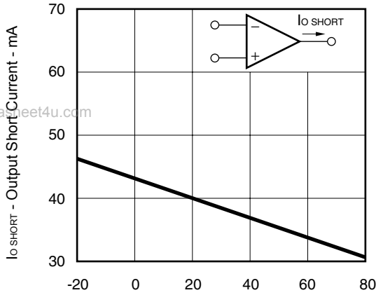
T_A - Operating Ambient Temperature - °C
