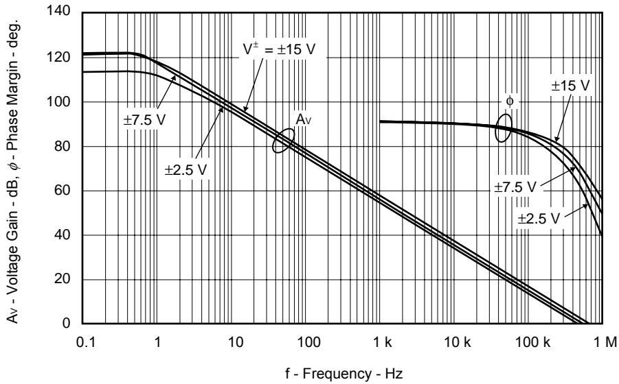
A_v, \phi vs. f
