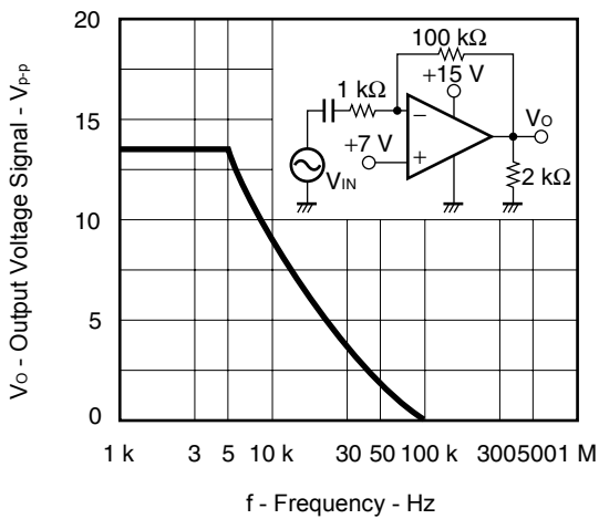
V_o vs. f
