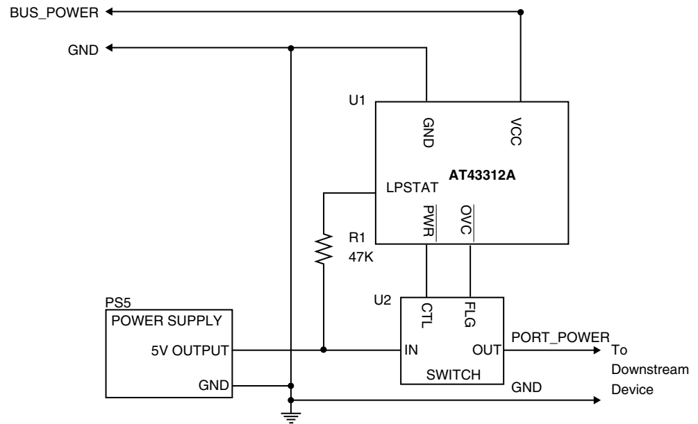
Figure 3. Bus Powered Hub Power Supply
