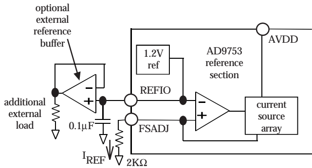
Figure 3. Internal Reference Configuration
