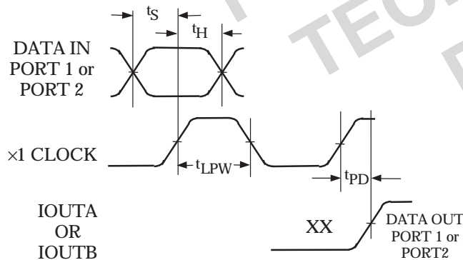
Figure 10. AD9753 Timing Requirements, Non-Interleaved Data with PLL Disabled
