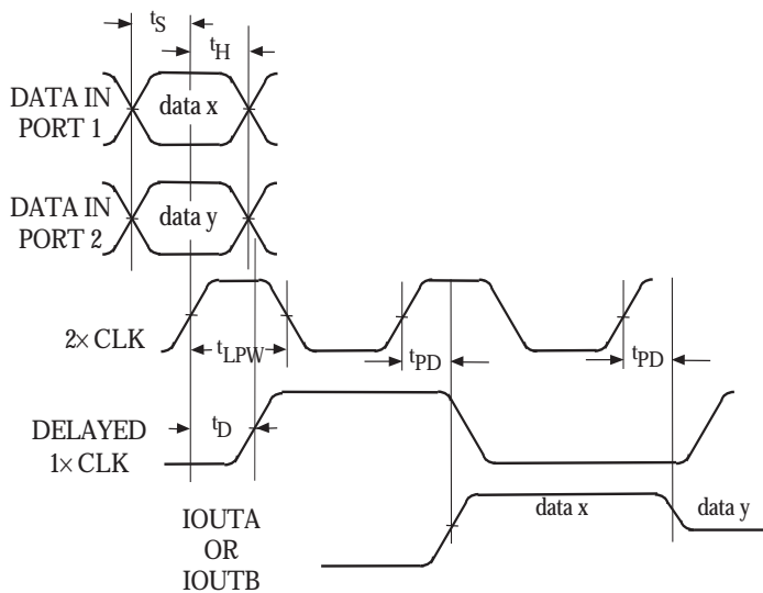
Figure 9. AD9753 Timing Requirements, Interleaving Data with PLL Disabled
