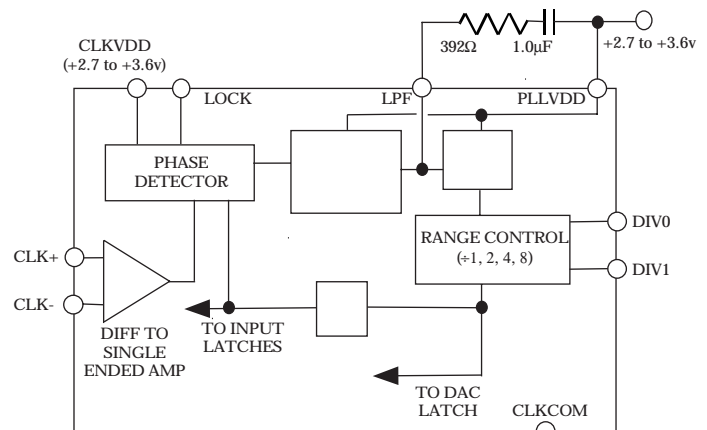
Figure 5. AD9753 Clock Circuitry with PLL Active
