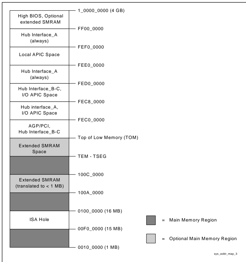
Figure 6. Detailed Extended Memory Range Address Map
