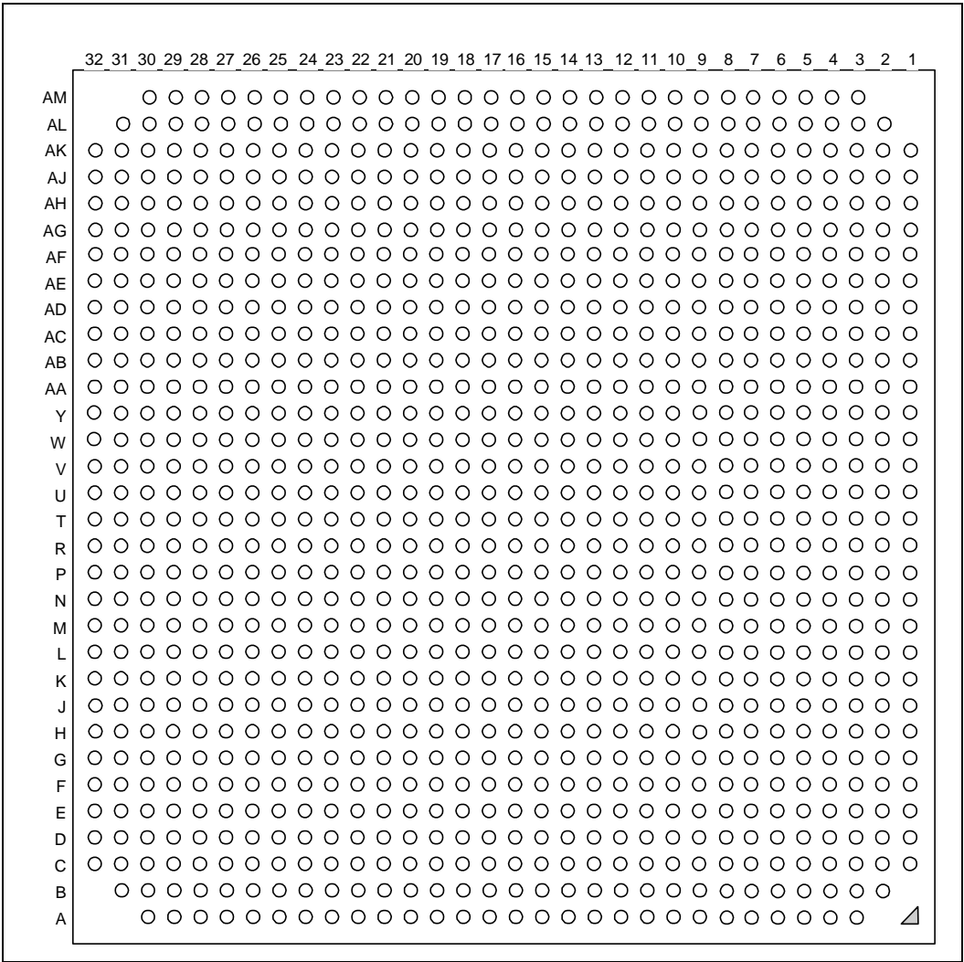
Figure 12. MCH Ballout Topside View (looking through the top of the package)
